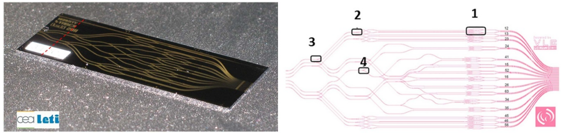
Figure 29. Left. Four-telescope beam-combiner of GRAVITY operating in K-band, designed and manufactured by photolithography of doped-silica on-silicon waveguides by CEA-LETI. Reproduced from [33], CC BY 4.0. Right. Design (by VLC Photonics-OCA based on [473]) of the SPICA six-telescope fringe-sensor operating in H band. Reproduced with permission from [474]. Each beam is divided in five equal parts thanks to a smart succession of 60/40 (3), 50/50 (2), and 66/33 (4) couplers. Each of the 15 possible pairs is combined inside an ABCD circuit (1), sampling the fringes with fixed phase shifts of 0, \pi/2 , \pi , and 3\pi/2 . This permits the instantaneous measurements of the phase-delay. Optical paths are equalized to avoid any bias in closure phase measurements.
