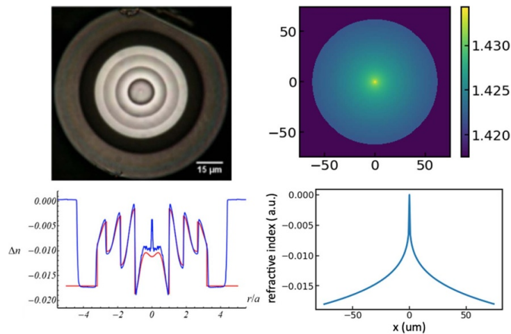
Figure 9. (top left) Optical micrograph of the Airy fiber (bottom left) physical refractive index profiles of the designed Airy (red), and of that of the PCVD preform (blue). Reproduced from I. Gris-Sánchez et al [161], (CC-BY 4.0). (top right) 2D theoretical refractive index profile of a fiber with logarithmic profile. (bottom right) 1D refractive index profile of the same fiber (relative to undoped silica). Reproduced from [161]. CC BY 4.0.
