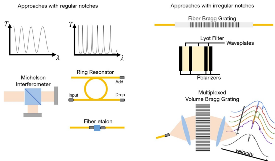
Figure 23. An overview of different ways to implement the optical correlation filter. The systems on the left create notches regularly spaced in frequency (diagrams at the top). The systems on the right create irregular notches by multi-step modulation. Figure 22 shows an example of irregular notches.
