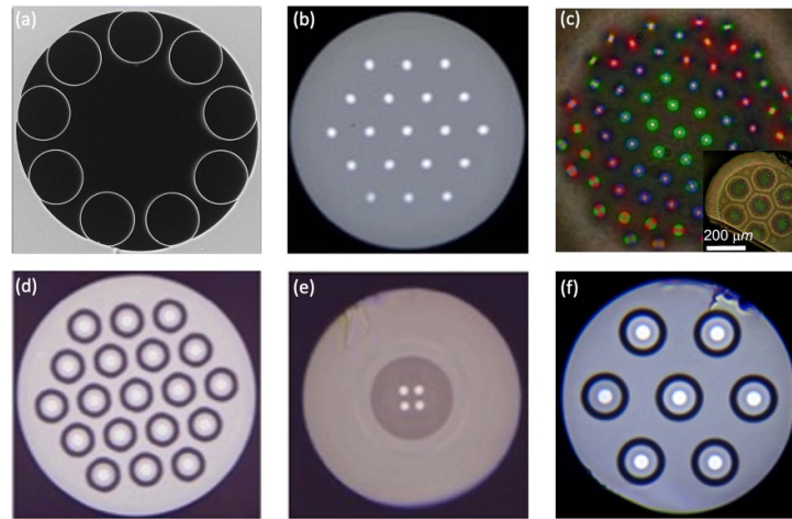
Figure 8. (a) Scanning electron image of an AR-HCF. The hollow-core is surrounded by an antiresonant cladding structure which consists of nine thin silica tubes. (b)–(f) Micrographs of multicore fibers featuring different index profiles and wavelength operation range.
