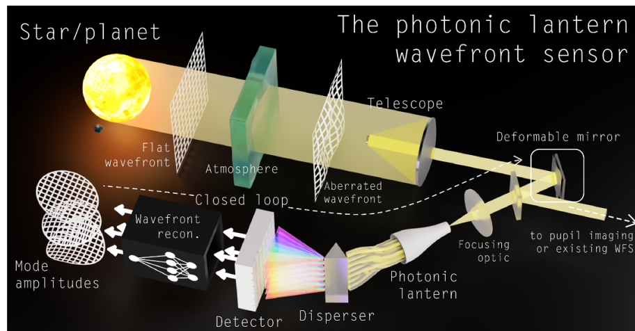
Figure 5. Overview of a PL-WFS system. Light arrives at the telescope distorted from the atmosphere. After the telescope mirrors, the light is guided to a photonic lantern, where it is distributed between different channels and exits at multiple outputs. Here, it can be spectrally dispersed and is then detected. The data can be used directly for scientific analysis as well as wavefront reconstruction (e.g. using a neural network), with the results feeding back to a deformable mirror earlier in the optics chain for wavefront correction.
