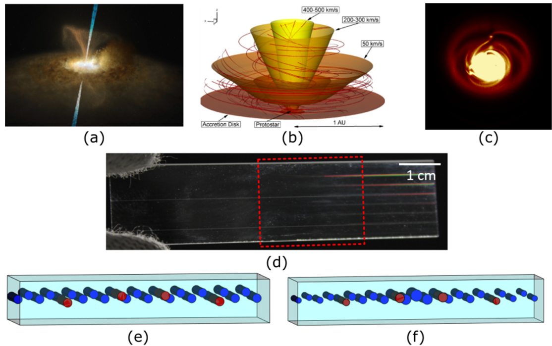
Figure 31. The science cases potentially addressable by a DBC-based interferometric combiner are shown in (a), (b) and (c). (a) Artist illustration of the environment around Active Galactic Nuclei (credit: ESO/M. Kornmesser and L. Calcada). (b) A model showing the magnetic field topology and velocity structure in the accretion region around a T Tauri star (credit: Romanova and Owocki). Reproduced with permission from [512]. (c) Radiative transfer simulations of a protoplanetary disk with embedded protoplanets, computed for wavelength of 10\ \mu\text{m} (credit: Kraus et al ). Reproduced with permission from [505]. (d) The IO chip used for on-sky tests at the William Herschel Telescope consists of pupil remappers, DBC (highlighted in red area) and coherent reformatters. Note that several DBC devices are contained in the red area (credit: AIP/A. Dinkelaker). (e) Design of current DBC with identical coupling coefficients across the width of the device. The red and blue cylinders are the input and output waveguides, respectively. (f) Design of a possible non-uniform DBC that has apodized coupling coefficients to enable broadband light measurements and precise estimation of visibilities.
