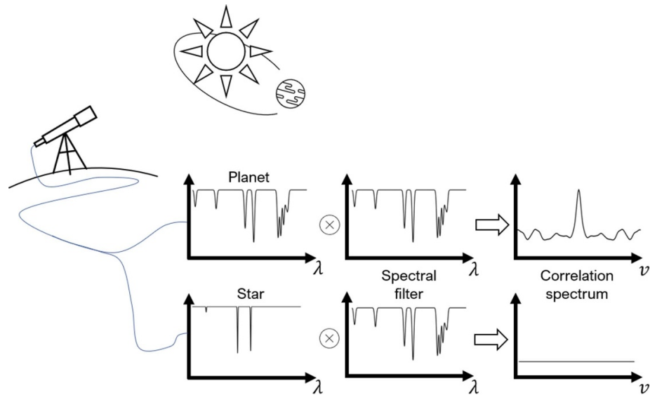
Figure 22. Light from two astrophysical sources (a star and a planet in this case) are fed to an optical cross-correlator spectrograph. The OSC passes the light of the objects through a spectral filter that is matched to a particular element in the planet's atmosphere. The planet has a strong correlation, while the star has no correlation signal at all. This allows the OCS to search for particular elements.
